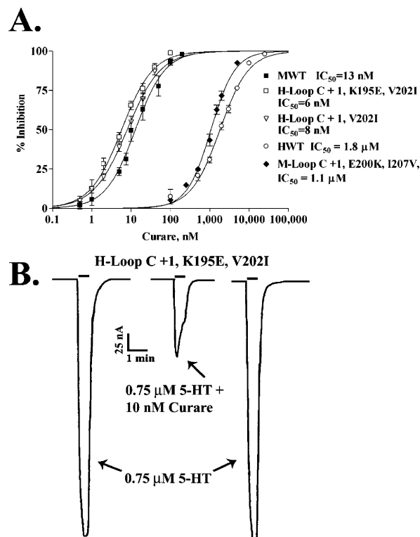
FIGURE 5: The combination of loop C+1 and two loop F receptor orthologs confer much of the curare potency of mouse and human 5-HT 3A receptors. In panel A, curare concentration response curves were generated in three chimeric receptors ( n = 4-10 ) and compared with that obtained in mouse WT and human WT (shown in Figure 2A). Gating concentrations of 5-HT, an EC 10 , were as follows: 1 \mu M, H-loop C+1, K195E, V202I; 0.75 \mu M, H-loop C+1, V202I; 1.75 \mu M, M-loop C+1, E200K, I207V. There are five more residues in the N-terminus of the mouse 5-HT 3A receptor than in that of the human 5-HT 3A receptor; human Lys195 and Val202 are the orthologs of mouse Glu200 and Ile207, respectively. One-way ANOVA of mouse WT, H-loop C+1, K195E, V202I, and H-loop C+1, V202I IC 50 's was not significant, p = 0.67 . In panel B, representative traces of 5-HT-mediated currents in the absence and presence of curare in H-loop C+1, K195E, V202I are displayed.
